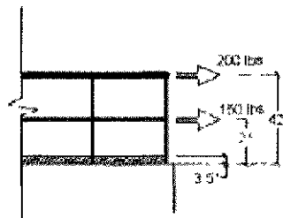
Figure J-1: Guardrail Requirements
